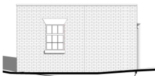
Kiosk - Proposed Southern Elevation
